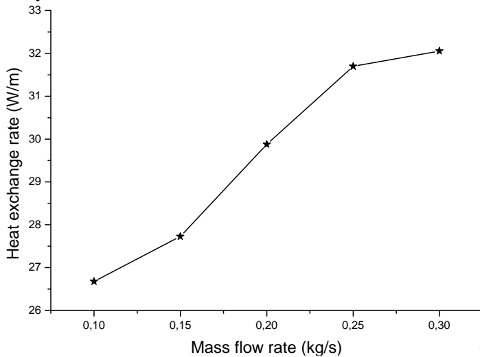
Fig.8. Heat exchange rate versus mass flow rate.
