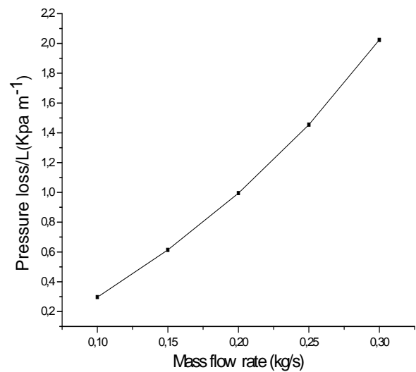
Fig.9. Pressure loss versus mass flow rate.
